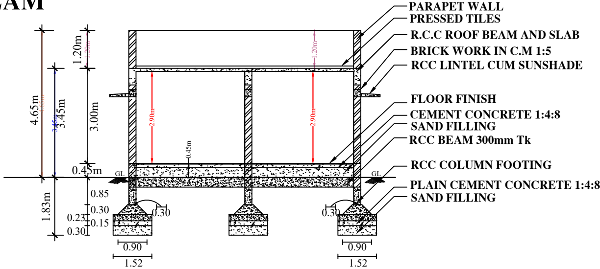
SECTION [A-A]
