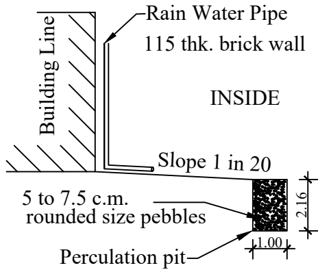
RAIN WATER HARVESTING PERCOLATION PIT
