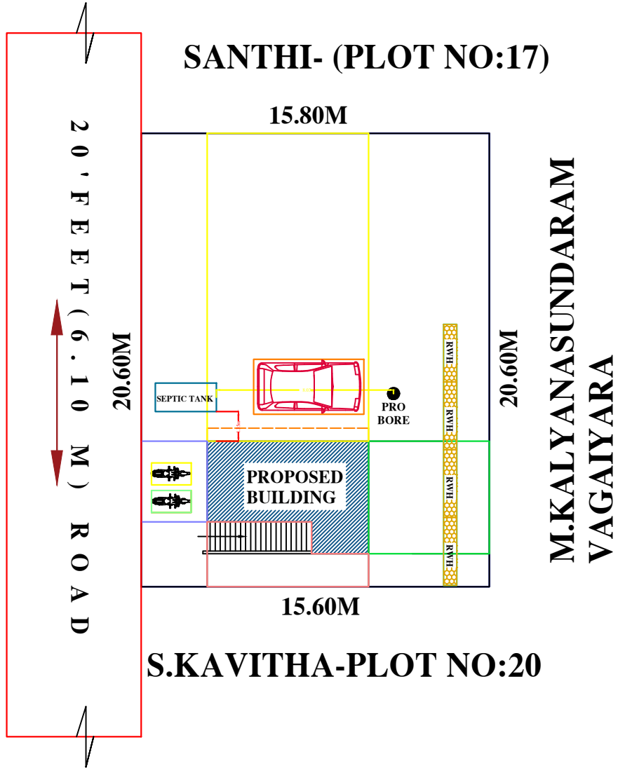
SITE PLAN
