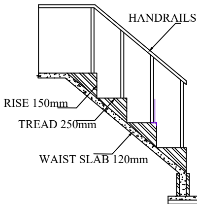
STAIRCASE DETAILS
