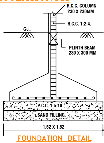
FOUNDATION DETAIL
