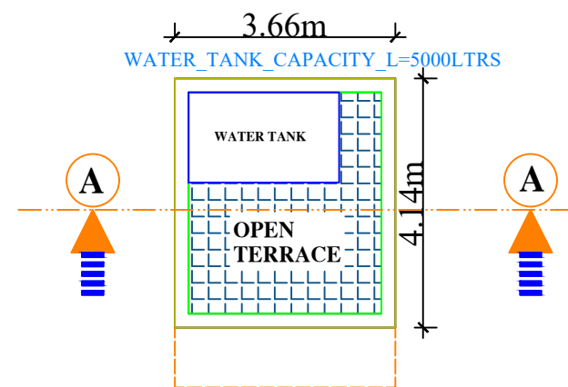
TERRACE PLAN
