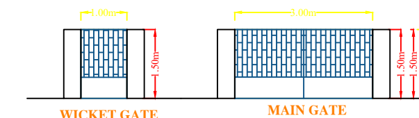
WICKET GATE
