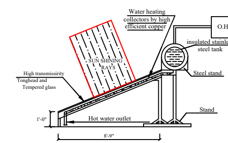
SECTION SOLAR WATER HEATER
