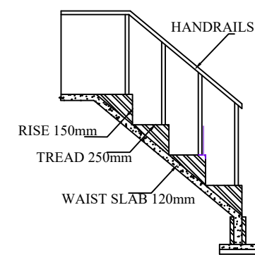
STAIRCASE DETAILS
