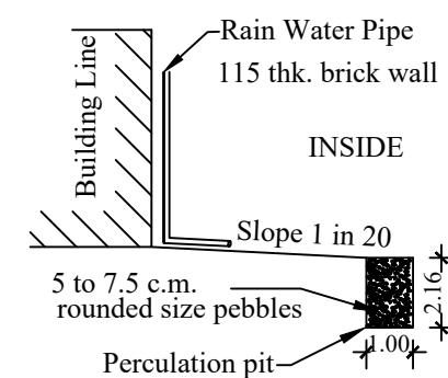
RAIN WATER HARVESTING PERCULATION PIT
