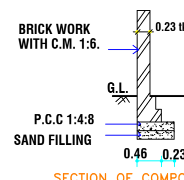
SECTION OF COMPOUND WALL
