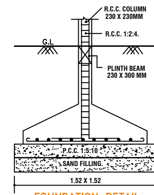
FOUNDATION DETAIL
