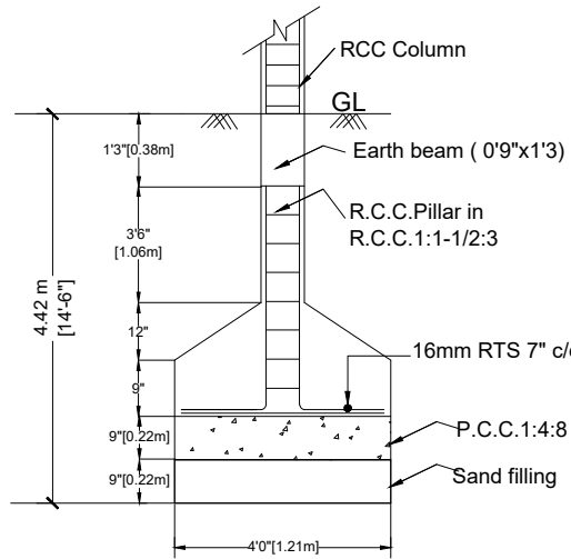
FOUNDATION DETAILS
