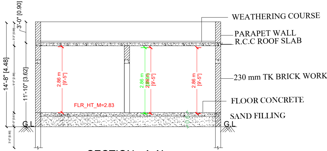
SECTION - A,A'
