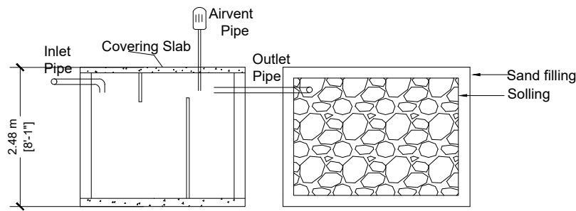
SECTION
