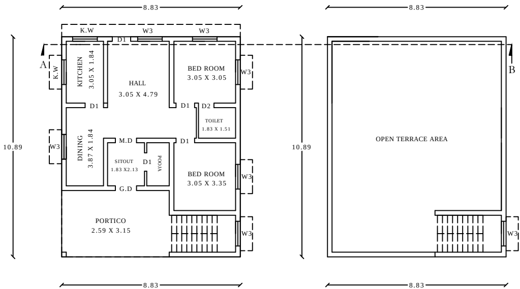
SECTION - "AB "
