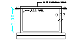
RWH SECTION (SAMPLE)
