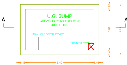
SUMP DETAIL SCALE 1\"/>
