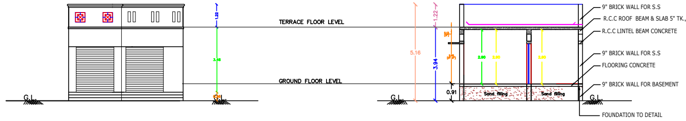
FRONT ELEVATION
