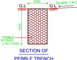
SECTION OF PEBBLE TRENCH
