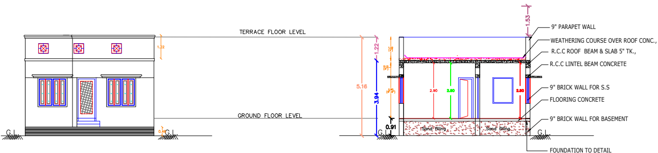
FRONT ELEVATION
