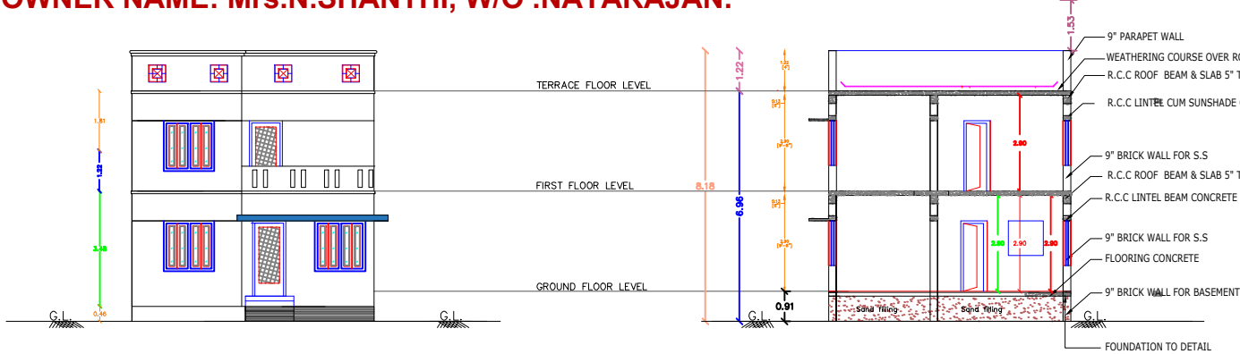
FRONT ELEVATION
