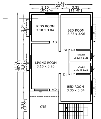
PRO. SECOND FLOOR PLAN
