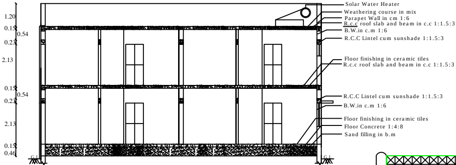
SECTION - "AB "
