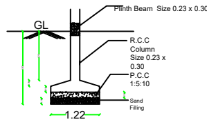
FOUNDATION DETAILS
