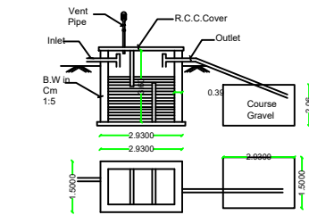
SEPTIC TANK & D-TRENCH DETAILS
