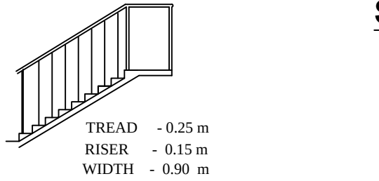
STAIRCASE DETAILS
