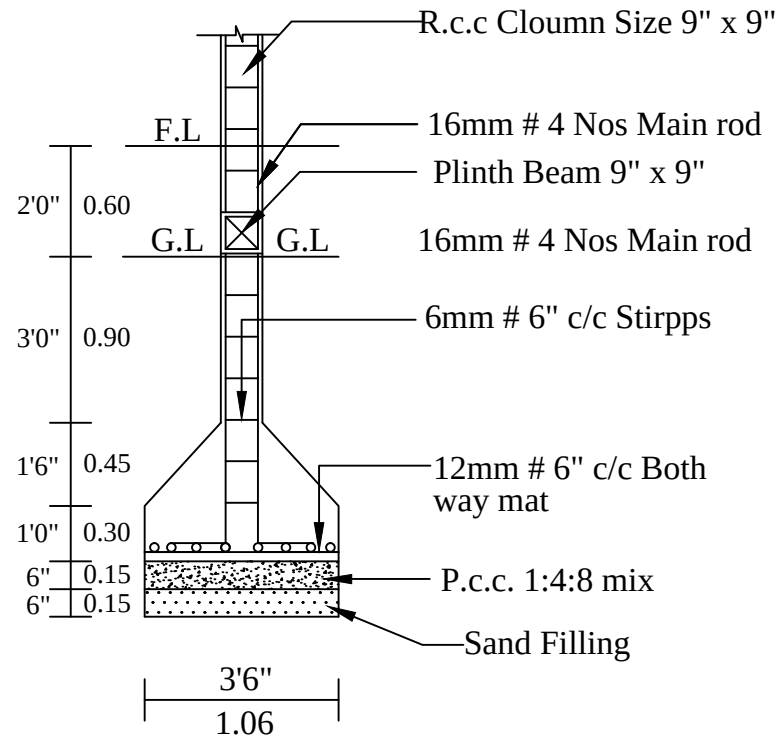
COLUMN DETIALS
