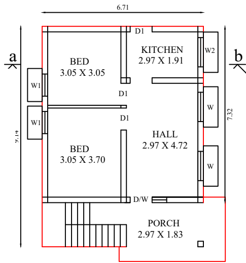
PROPOSED PLAN
