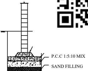
COLUMN DETAILS
