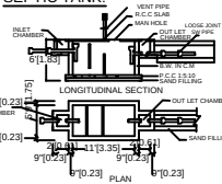
SEPTIC TANK:
