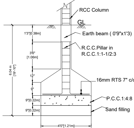
FOUNDATION DETAILS
