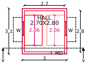
PRO.GROUND FLOOR PLAN
