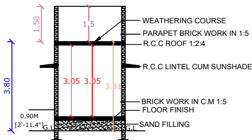
SECTION ON XX
