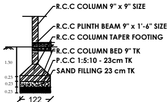
SECTION COLUMN DETAILS PLAN
