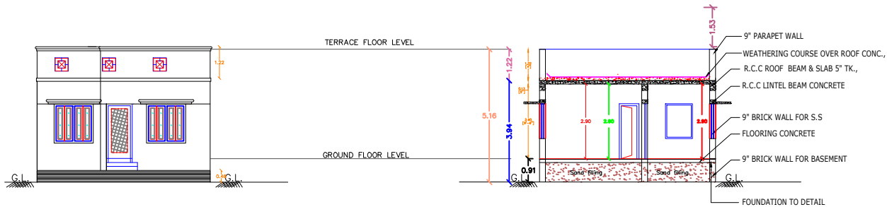
FRONT ELEVATION
