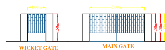
WICKET GATE
