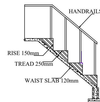
STAIRCASE DETAILS
