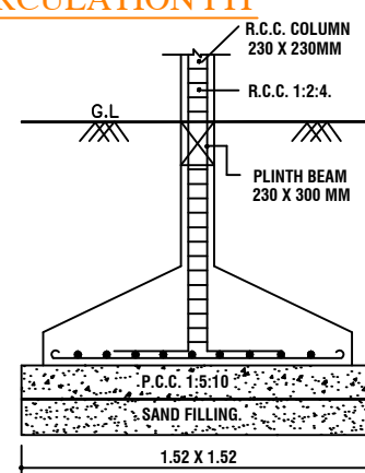
FOUNDATION DETAIL
