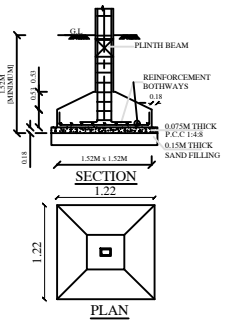
FOUNDATION DETAILS
