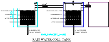
RAIN WATER COLL. TANK
