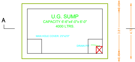
SUMP DETAIL SCALE 1"=4'0"
