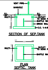
PLAN SEPTIC TANK
