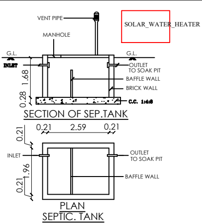
SECTION OF SEPTIC TANK
