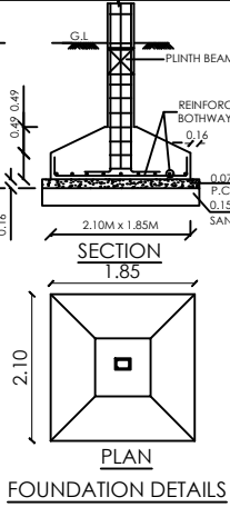
FOUNDATION DETAILS
