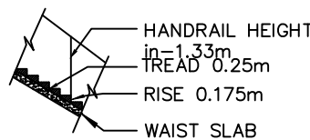
STAIRCASE DETAILS
