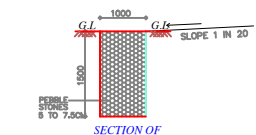
SECTION OF PEBBLE TRENCH
