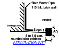
RAIN WATER PIPE
