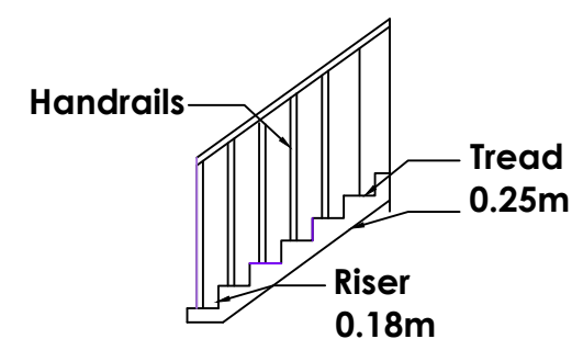
STAIRCASE DETAILS
