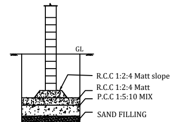
COLUMN DETAILS
