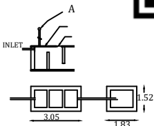
DETAILS OF SEPTIC TANK & DISPERSION TRENCH
