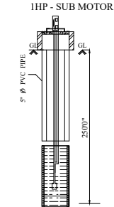
BOREWELL DETAILS
