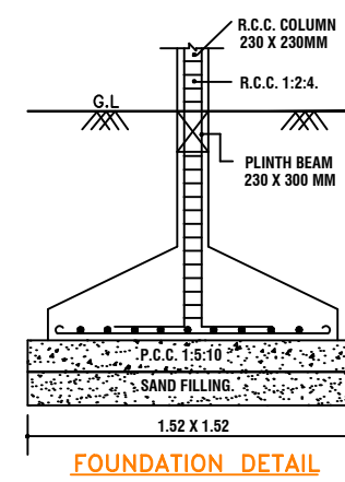
FOUNDATION DETAIL
