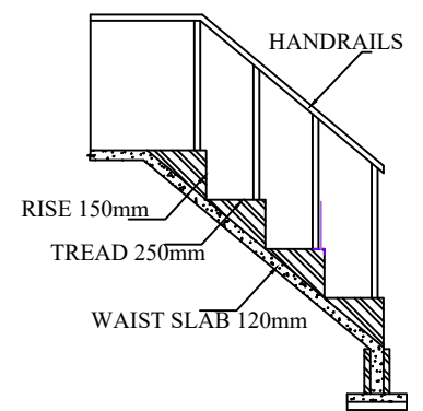
STAIRCASE DETAILS
