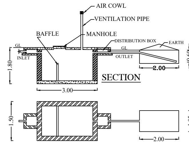
SEPTIC TANK DISPERSION TRENCH
