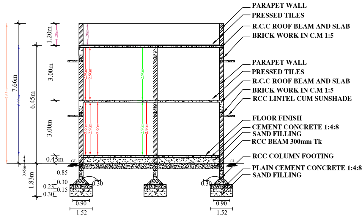
SECTION [A-A]
