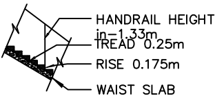
STAIRCASE DETAILS
