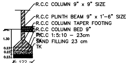
SECTION PLAN COLUMN DETAILS
