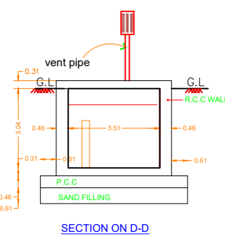
SECTION ON D-D
