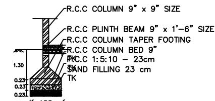
SECTION COLUMN DETAILS PLAN
