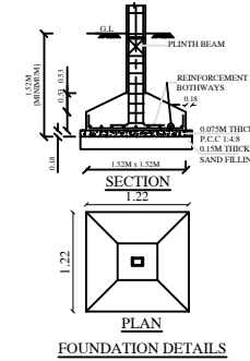
PLAN FOUNDATION DETAILS
