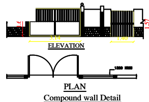
PLAN Compound wall Detail
