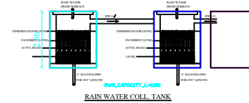
RAIN WATER COLL. TANK
