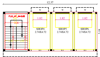
FLOOR PLAN
