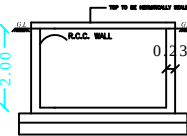
MAIN GATE ELEVATION
