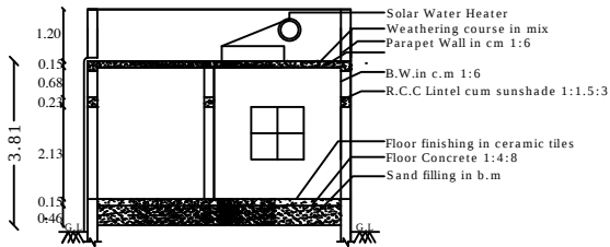
SECTION - "AB "
