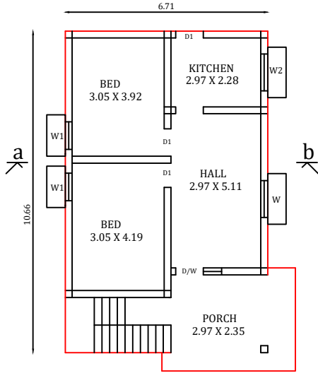
PROPOSED PLAN
