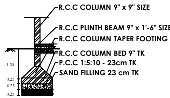
SECTION
