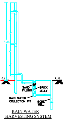
RAIN WATER HARVESTING SYSTEM
