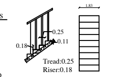
STAIRCASE DETAIL
