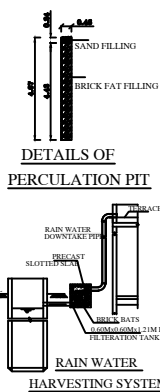
RAIN WATER HARVESTING SYSTEM
