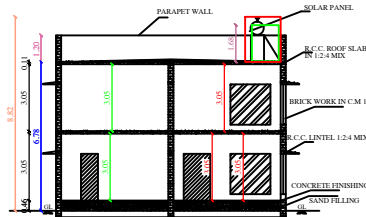
SECTION ON - BB (BLOCK - 2)
