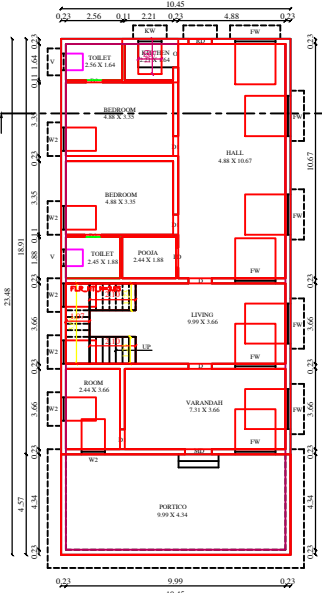
GROUND FLOOR PLAN (BLOCK - 2)
