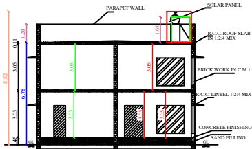
SECTION ON - AA (BLOCK - 1)
