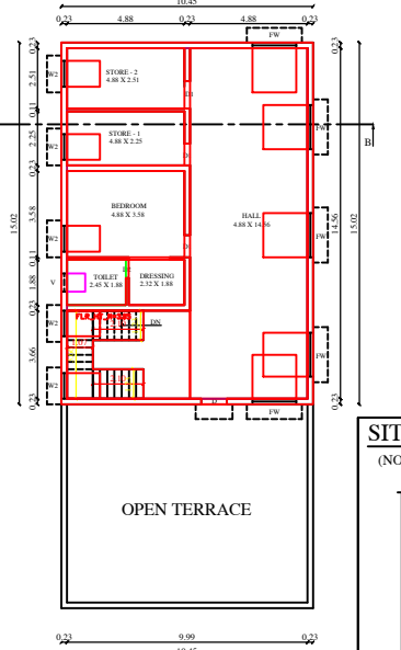
FIRST FLOOR PLAN (BLOCK - 2)
