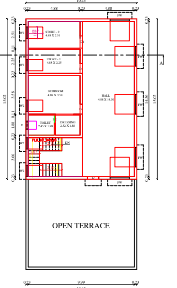
FIRST FLOOR PLAN (BLOCK - 1)
