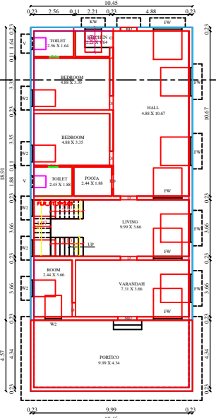
GROUND FLOOR PLAN (BLOCK - 1)
