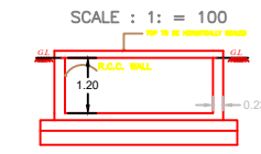
RWH SECTION (SAMPLE) RWHP_CAPACITY_L = 2000LTRS
