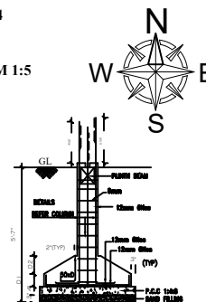
FOUNDATION DETAILS
