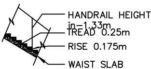
AIRCASE DETAILS
