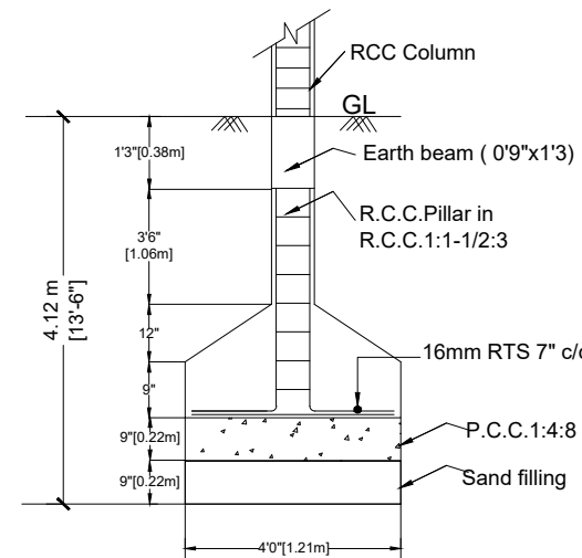
FOUNDATION DETAILS
