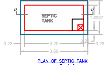
PLAN OF SEPTIC TANK
