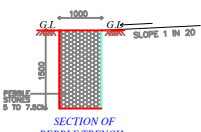
SECTION OF PEBBLE TRENCH
