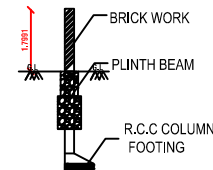
BRICK WORK SECTION
