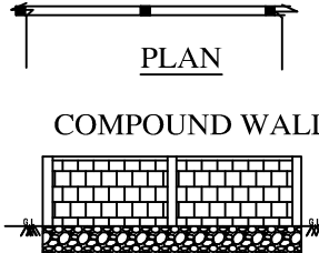
COMPOUND WALL ELEVATION
