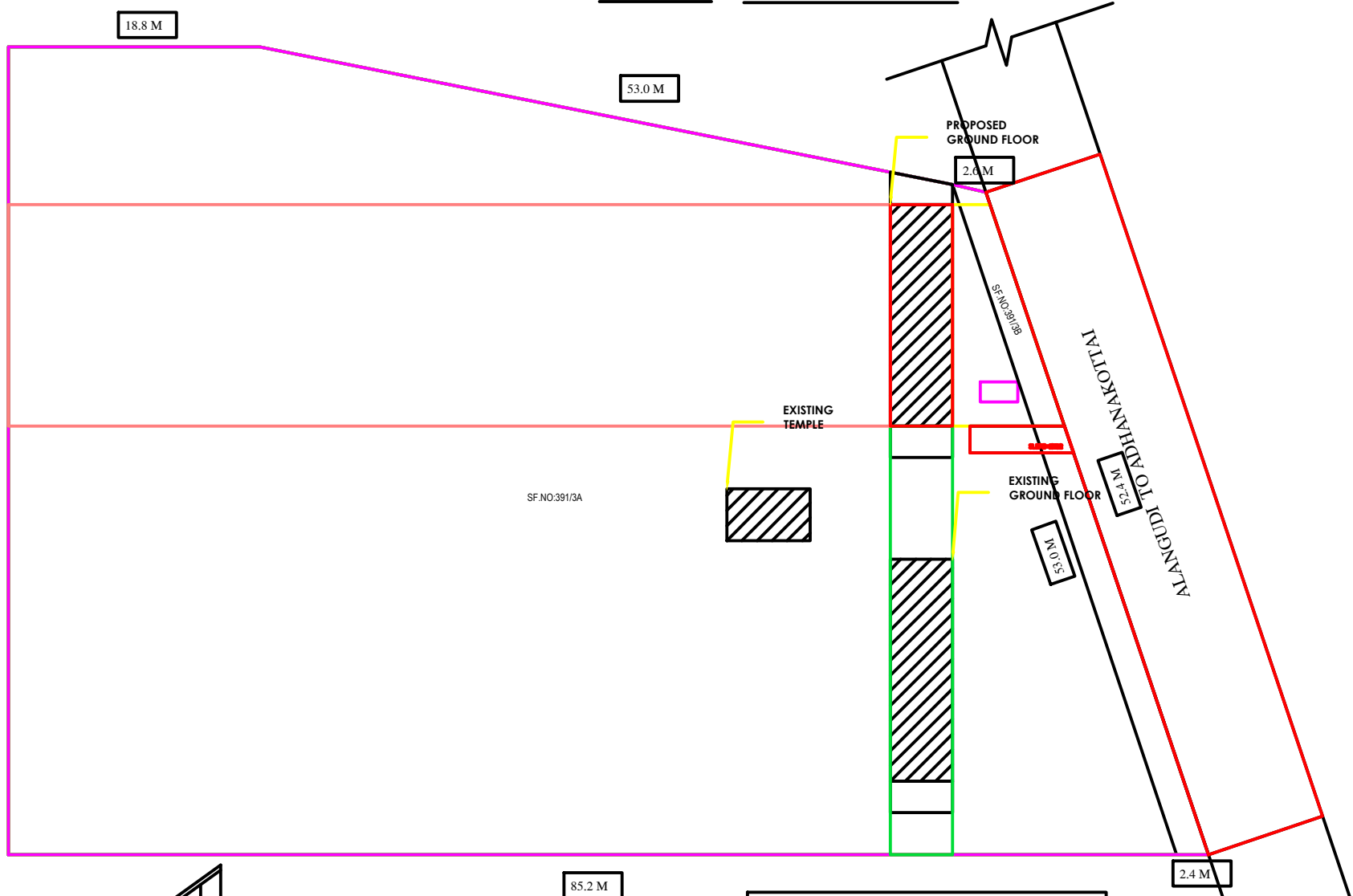
SECTION-AA SITE PLAN
