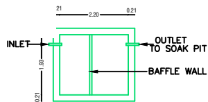
PLAN SEPTIC. TANK
