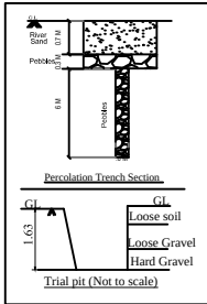
FOUNDATION DETAILS
