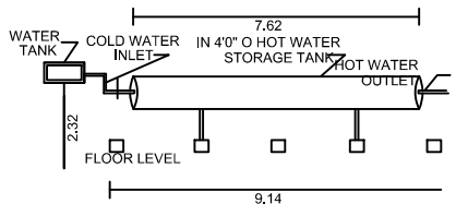
SOLAR HOT WATER SYSTEM DETAILS
