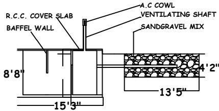
SEPTIC TANK AND DISPERSION TRENCH DETAILS
