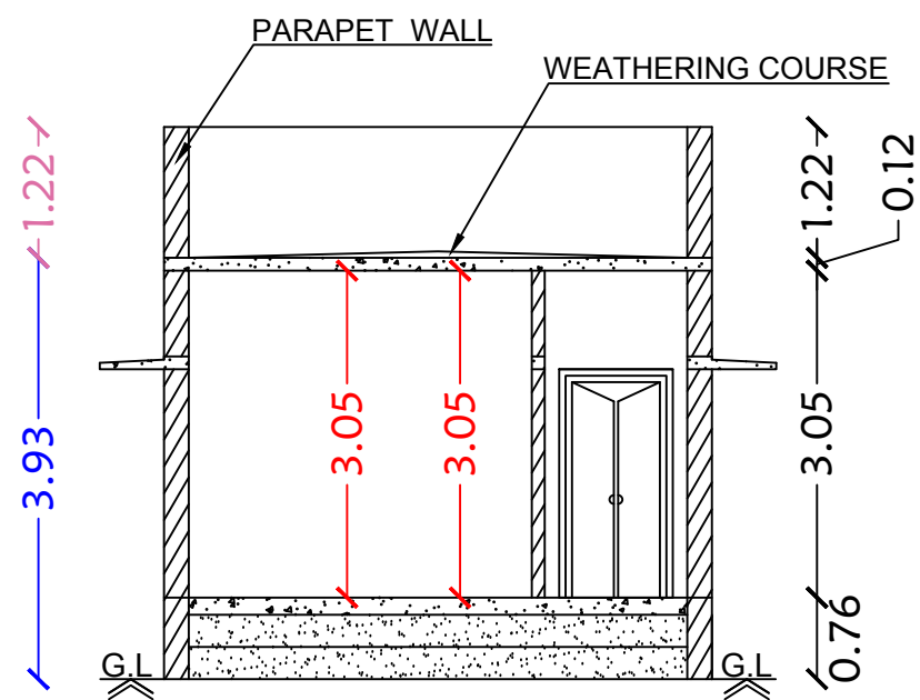
Section on-"AA"
