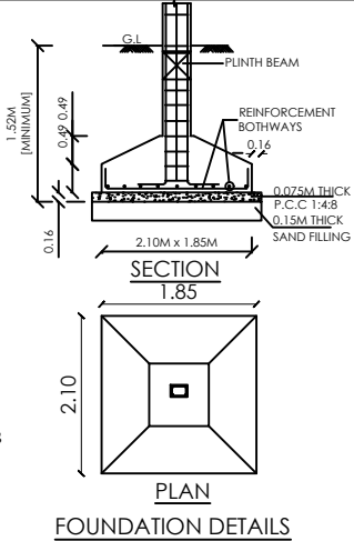
FOUNDATION DETAILS
