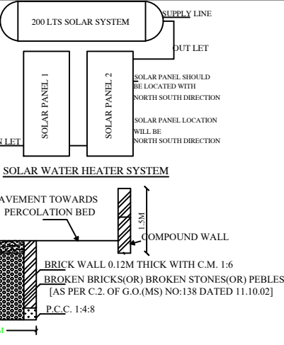
SECTION OF RAIN WATER PERCOLATION BED
