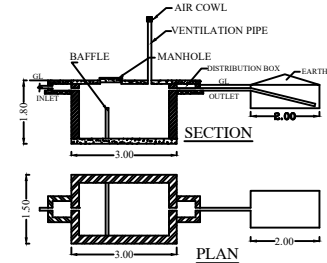
SEPTIC TANK DISPERSION TRENCH
